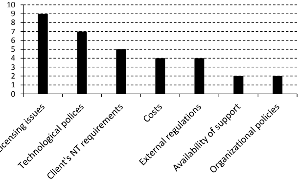
Figure 2. Non-technical NFRs.
