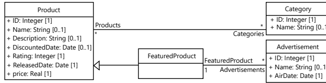
Fig. 1. UML class diagram of the running example.
