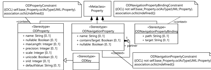
Fig. 3. Properties and associations stereotypes.
