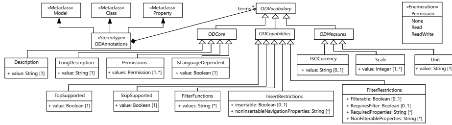
Fig. 4. Annotation and vocabulary stereotypes.
